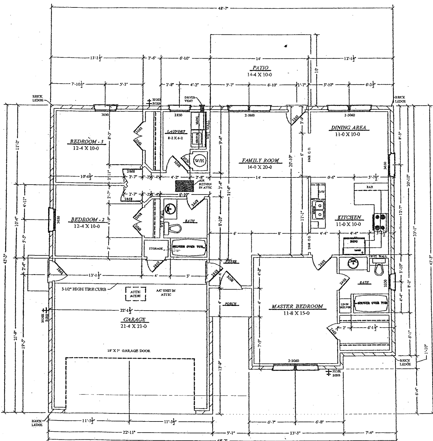
FLOOR PLAN
